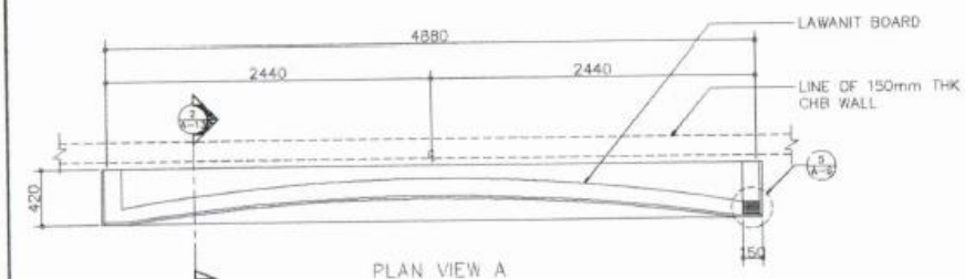
BLACKBOARD DETAIL SCALE 1:20 M.
