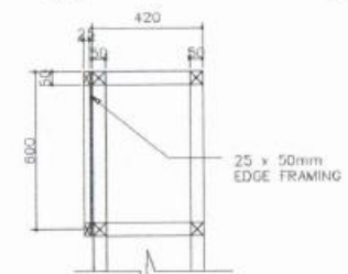
SPOT DETAIL SECTION EDGE FRAMING SCALE 1:10 M.
