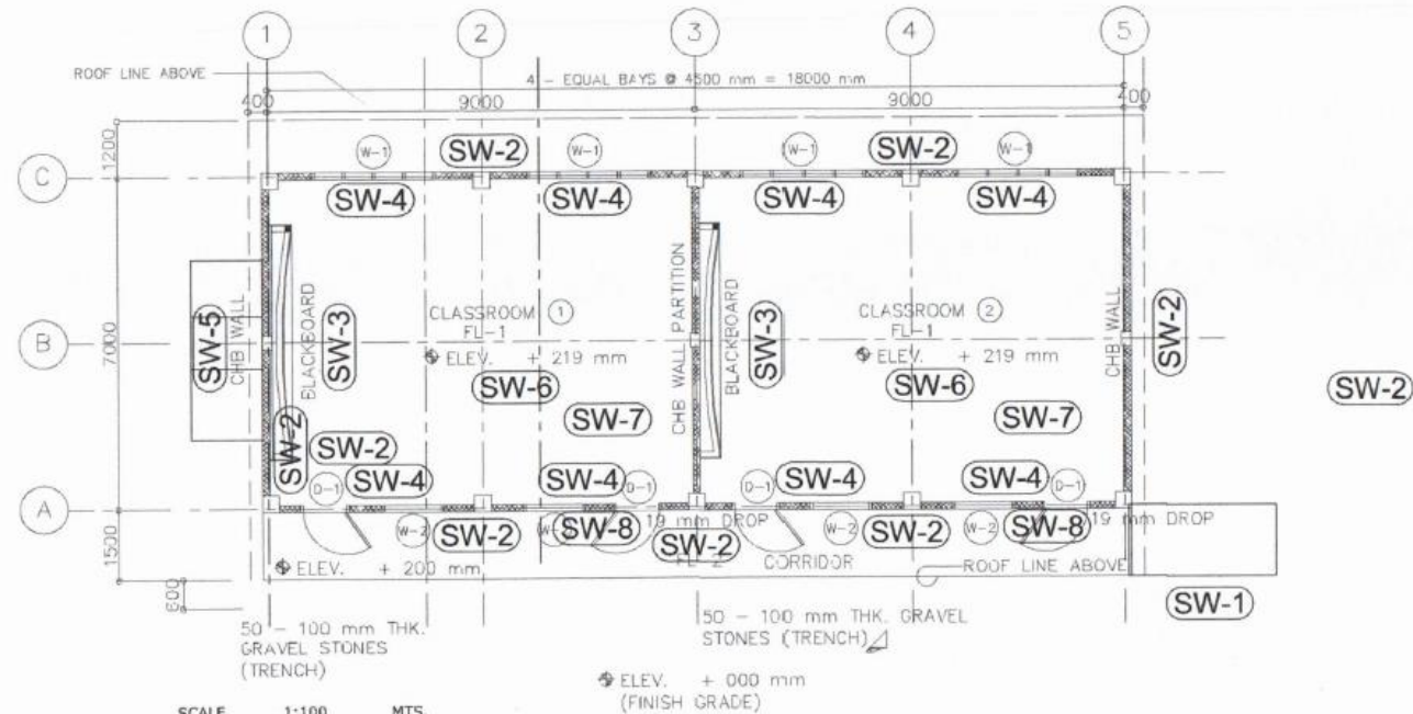
FLOOR PLAN
