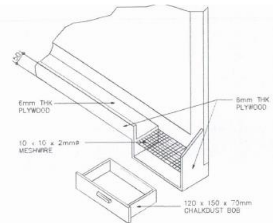
CHALK DUST BOX DETAIL SCALE 1:15 M.
